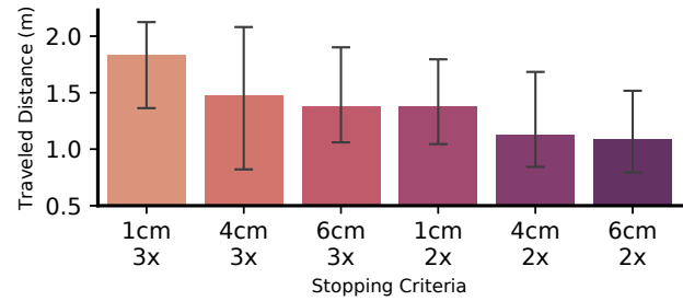
Figure 9: Stopping Criteria. The figure plots the median traveled distance for different stopping criteria. Error bars denote the 10 th and 90 th percentile.
